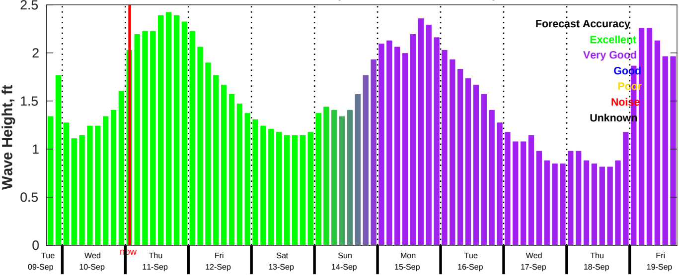
CMEMS Wave Forecast for NDBC 42035 from 09-Sep-2025 18:00:00 to 19-Sep-2025 18:00:00
