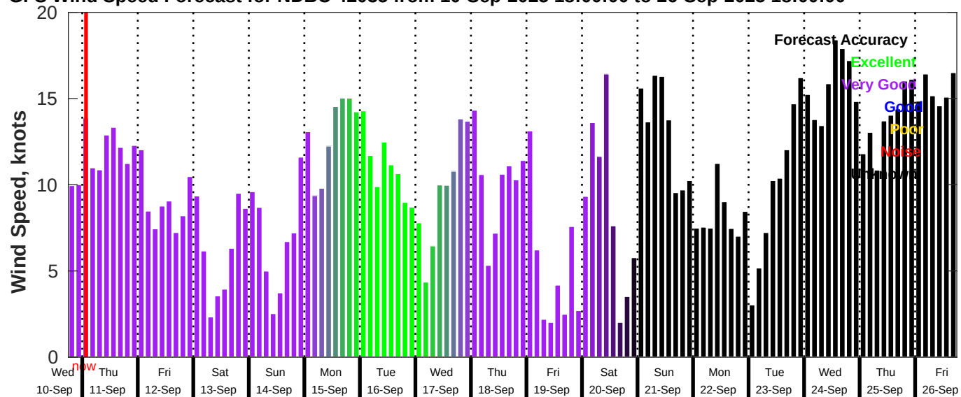
GFS Wind Speed Forecast for NDBC 42035 from 10-Sep-2025 18:00:00 to 26-Sep-2025 18:00:00
