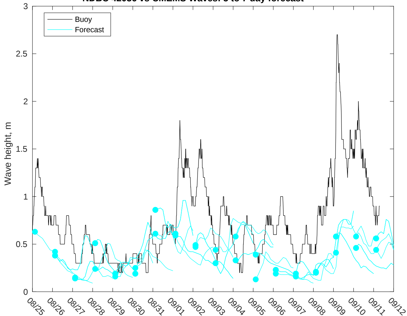
NDBC 42036 vs CMEMS Waves: 5 to 7 day forecast
