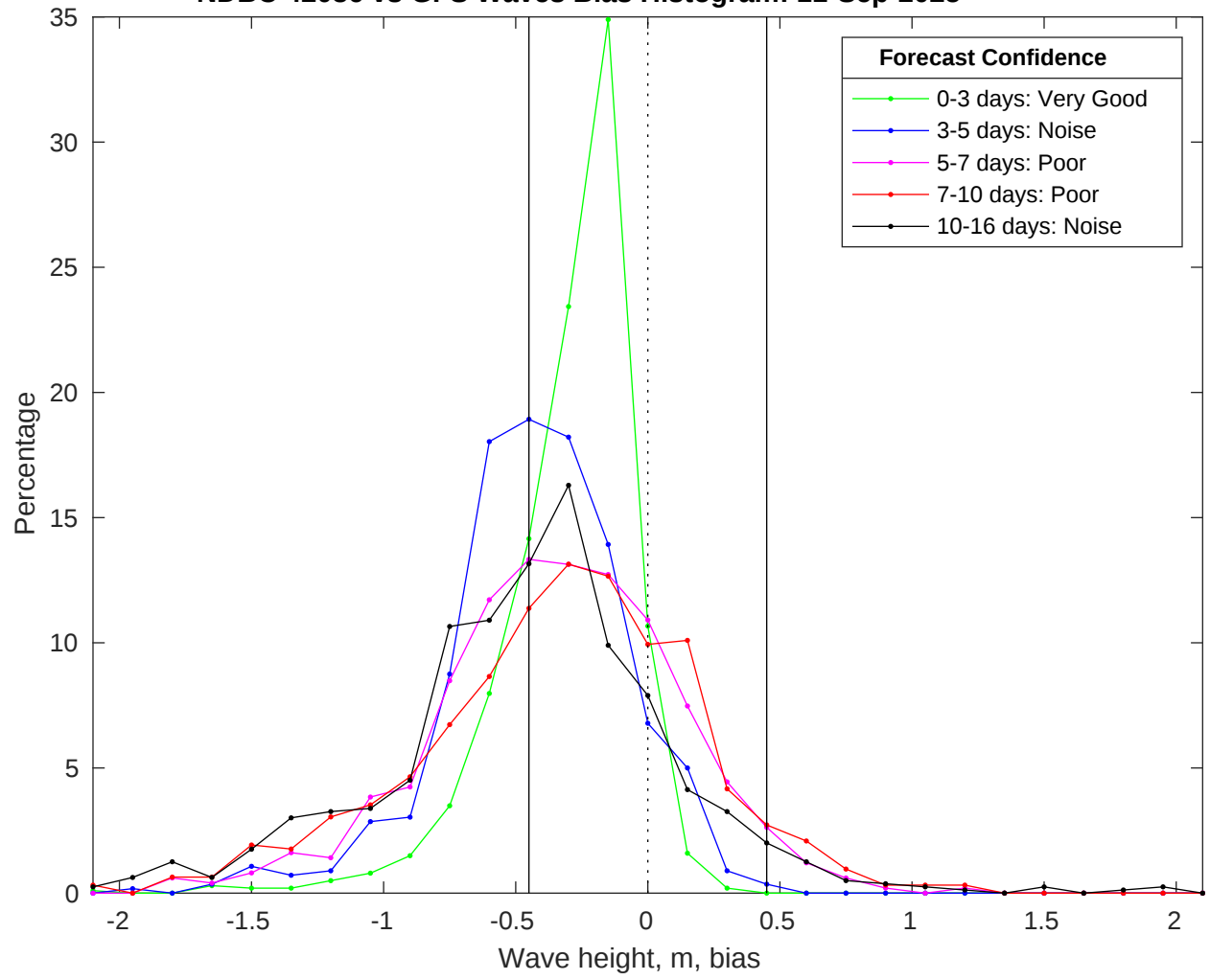
NDBC 42036 vs GFS Waves Bias Histogram: 11-Sep-2025
