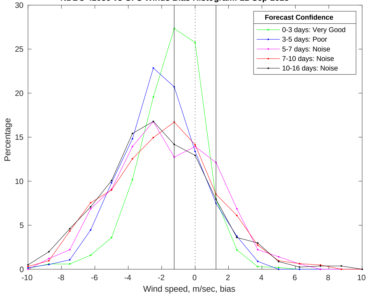
NDBC 42036 vs GFS Winds Bias Histogram: 11-Sep-2025
