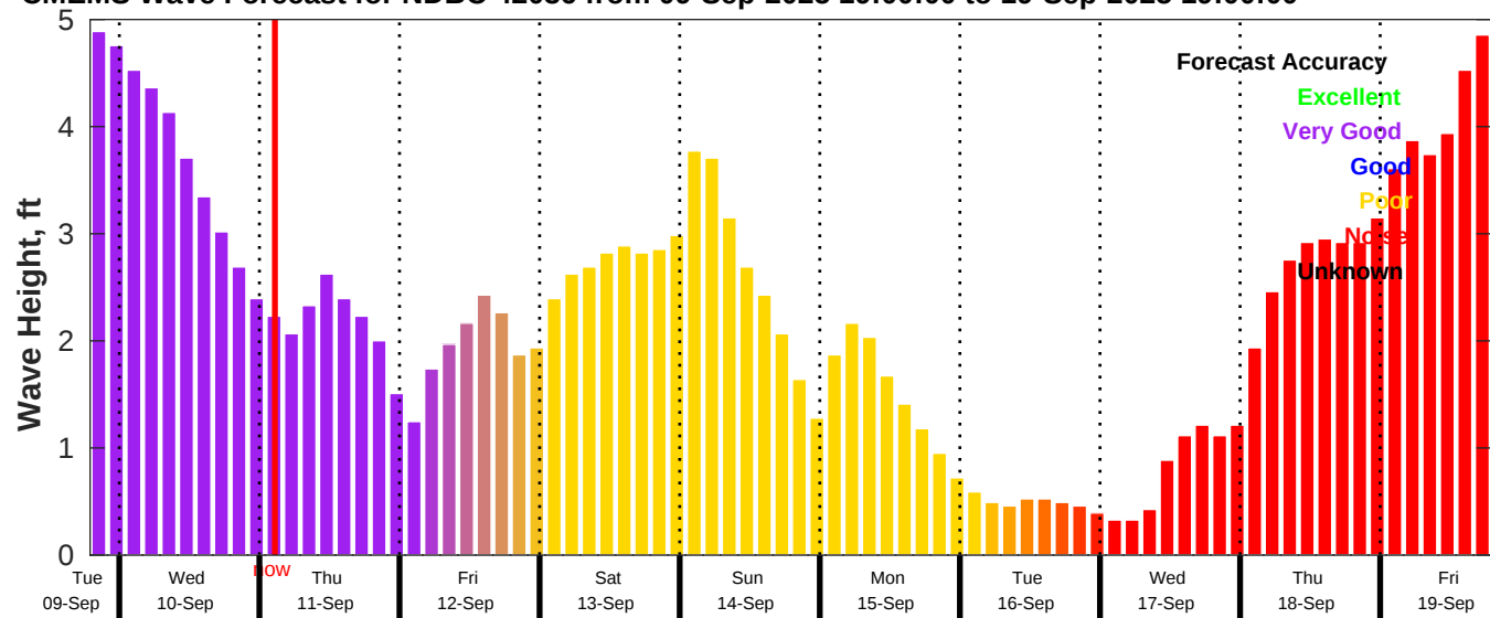
CMEMS Wave Forecast for NDBC 42036 from 09-Sep-2025 19:00:00 to 19-Sep-2025 19:00:00
