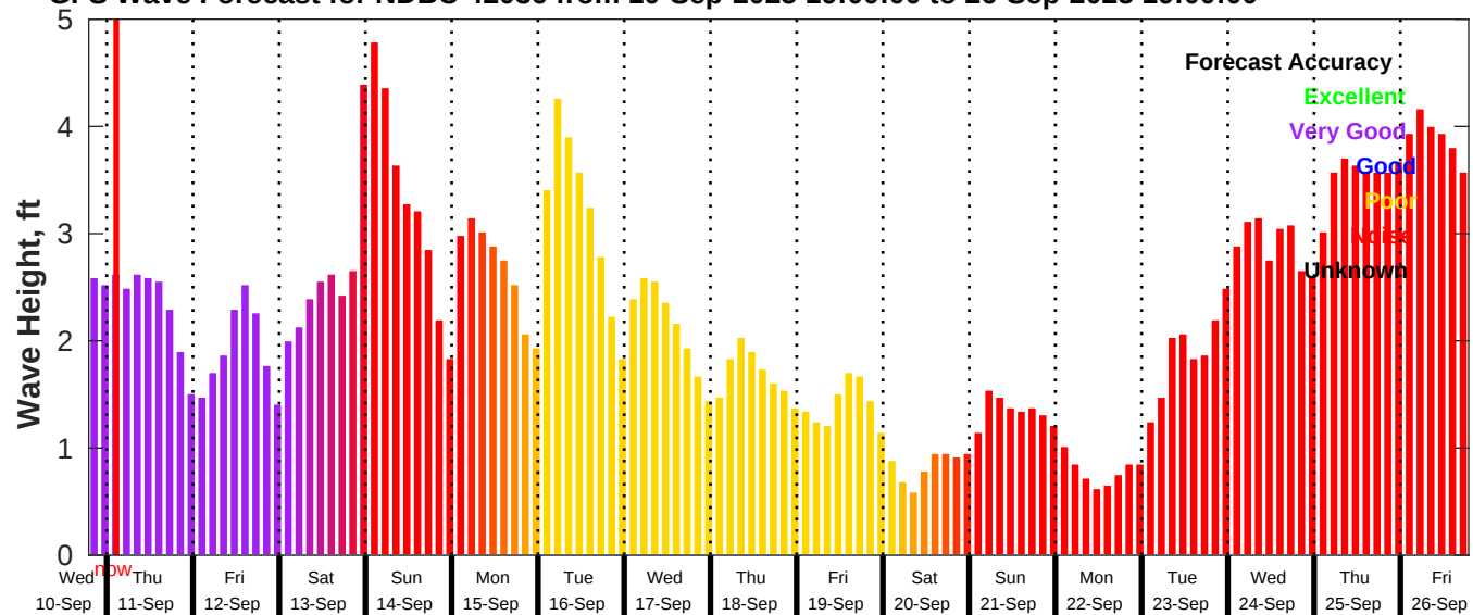
GFS Wave Forecast for NDBC 42036 from 10-Sep-2025 19:00:00 to 26-Sep-2025 19:00:00
