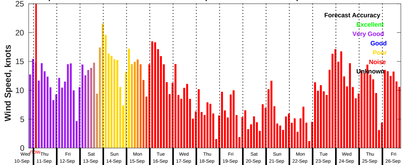
GFS Wind Speed Forecast for NDBC 42036 from 10-Sep-2025 19:00:00 to 26-Sep-2025 19:00:00
