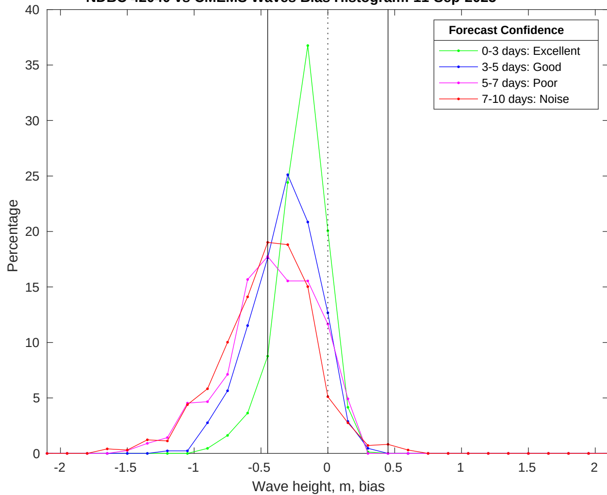
NDBC 42040 vs CMEMS Waves Bias Histogram: 11-Sep-2025
