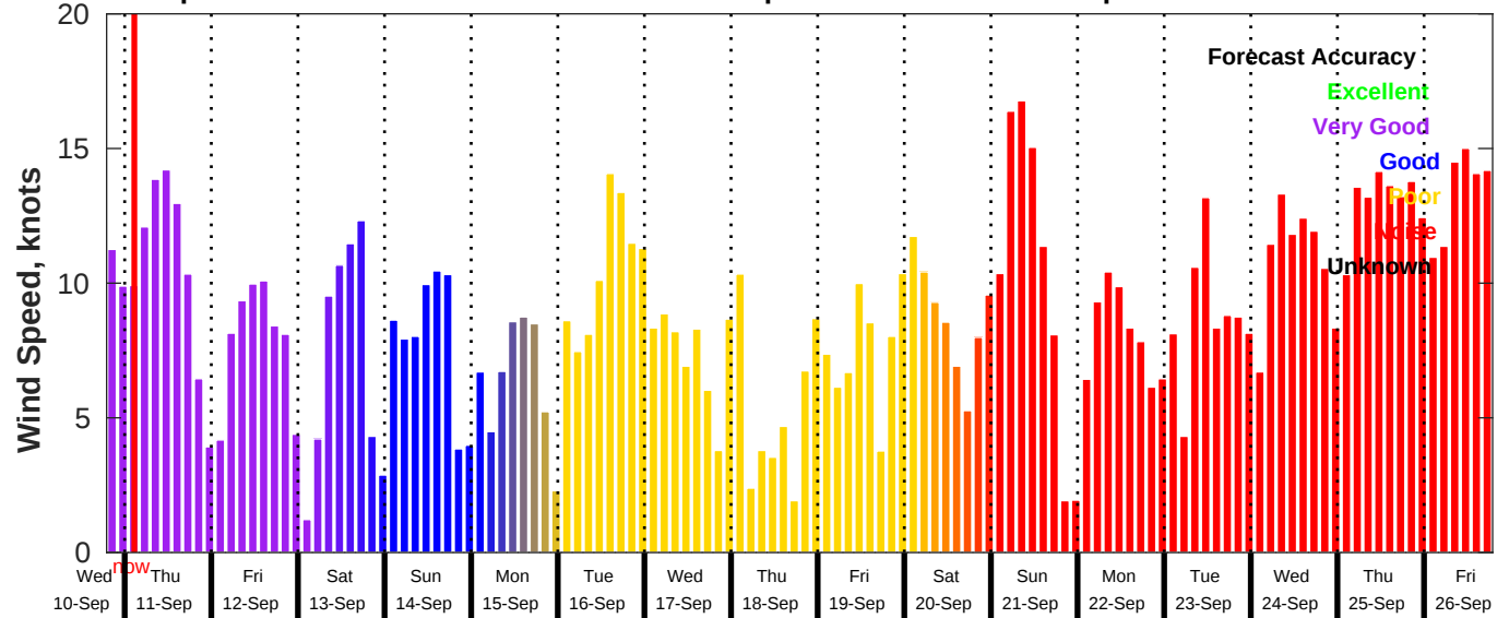
GFS Wind Speed Forecast for NDBC 42040 from 10-Sep-2025 19:00:00 to 26-Sep-2025 19:00:00
