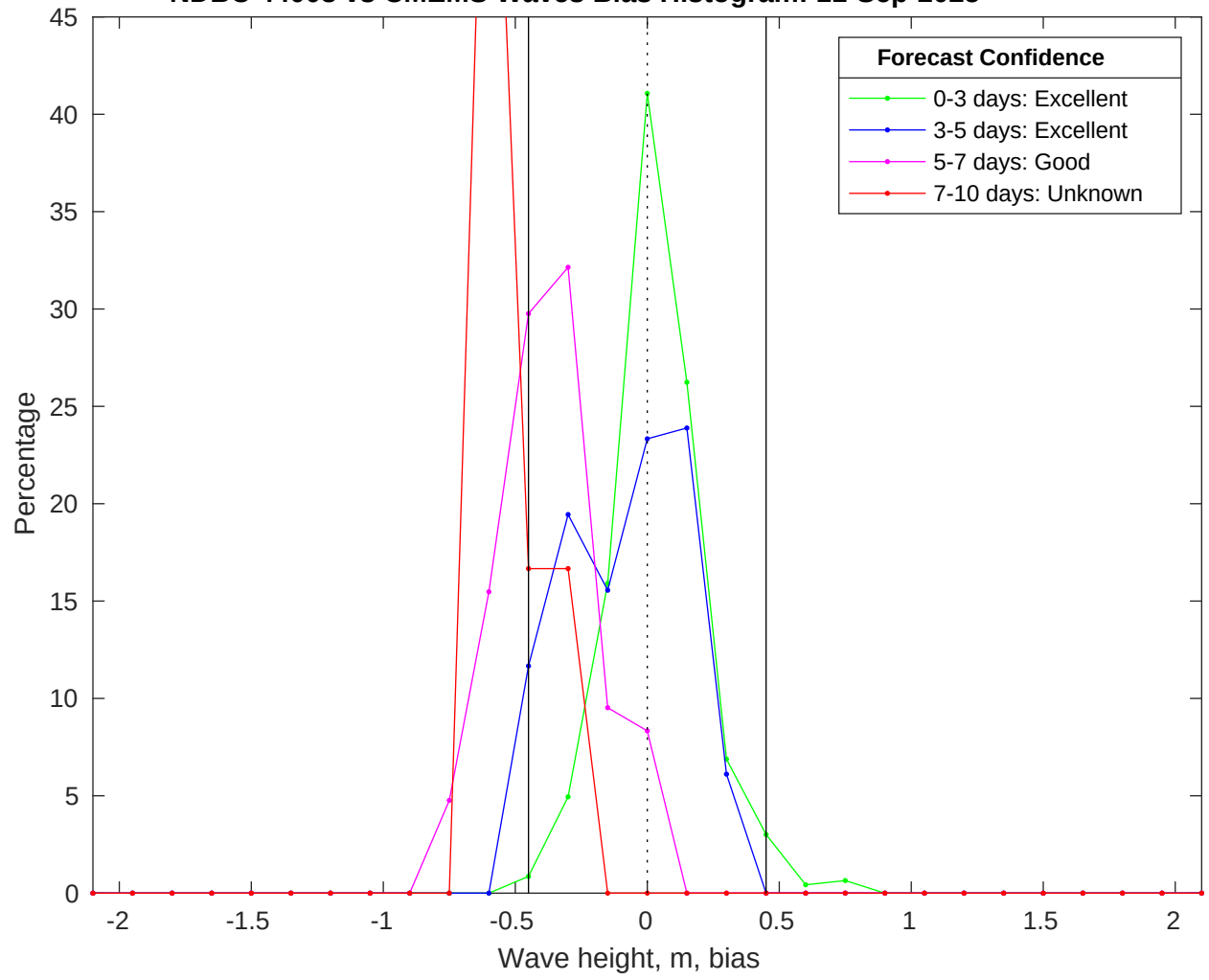
NDBC 44008 vs CMEMS Waves Bias Histogram: 11-Sep-2025
