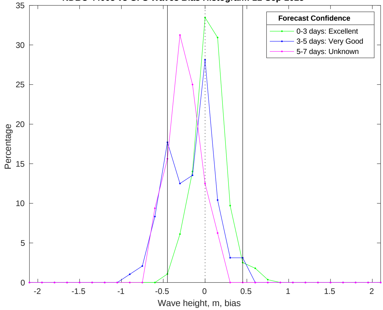
NDBC 44008 vs GFS Waves Bias Histogram: 11-Sep-2025
