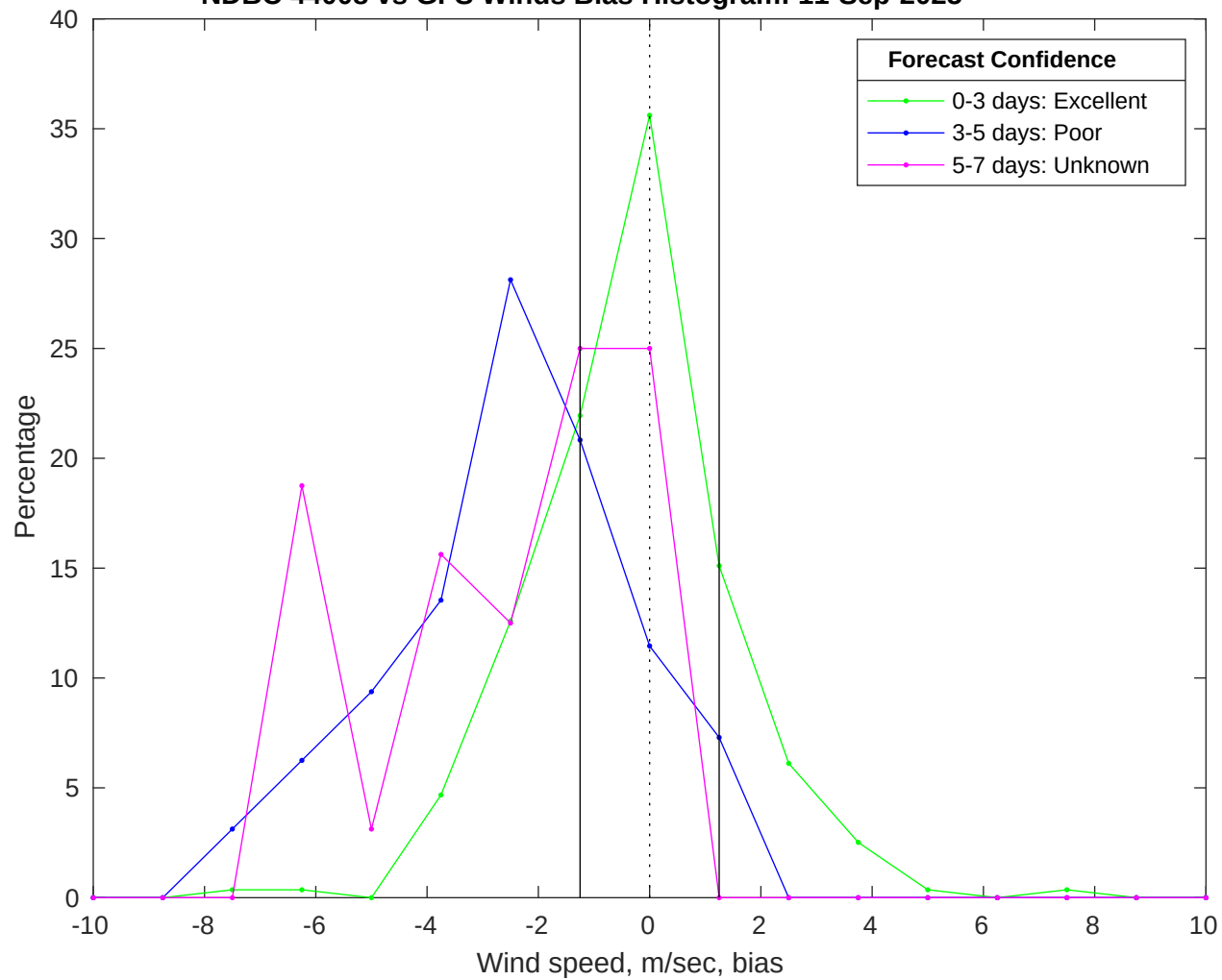
NDBC 44008 vs GFS Winds Bias Histogram: 11-Sep-2025
