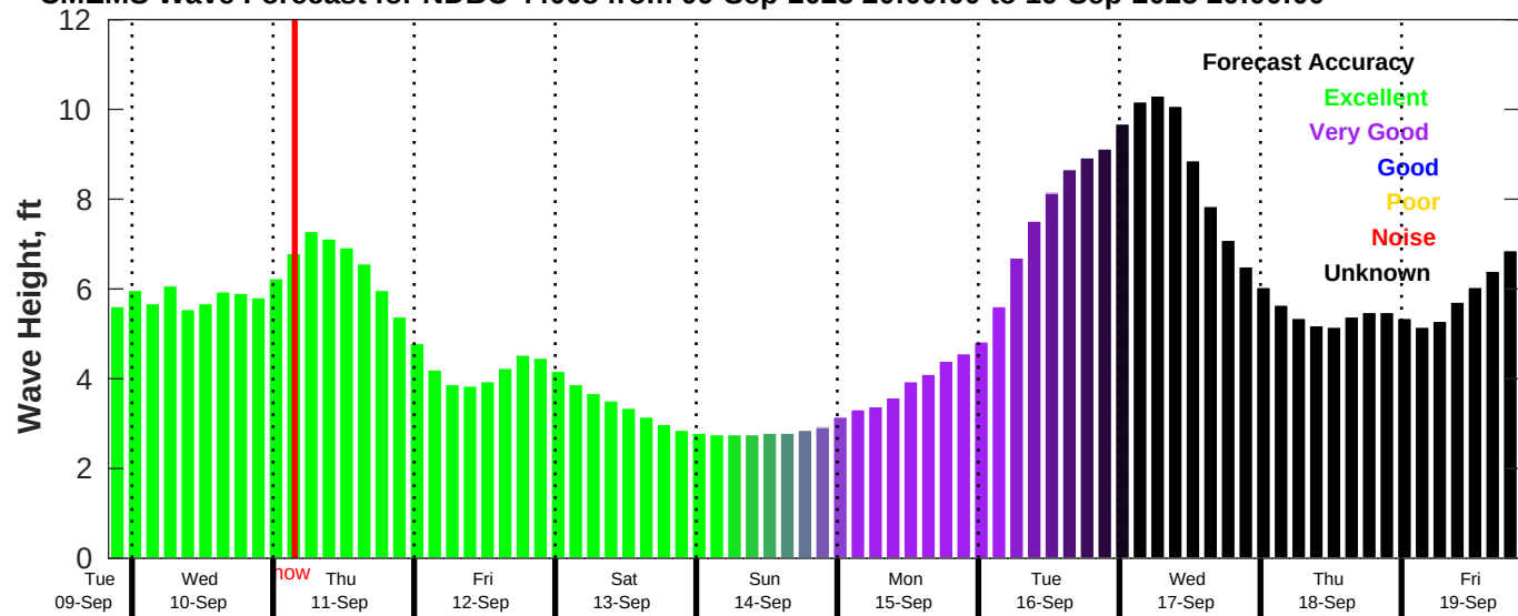
CMEMS Wave Forecast for NDBC 44008 from 09-Sep-2025 20:00:00 to 19-Sep-2025 20:00:00
