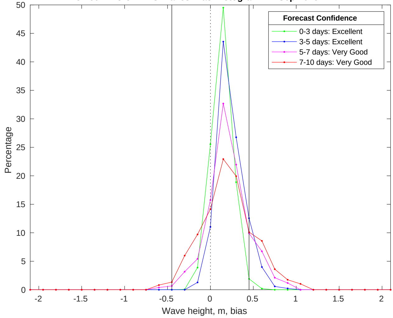
NDBC 46011 vs CMEMS Waves Bias Histogram: 11-Sep-2025
