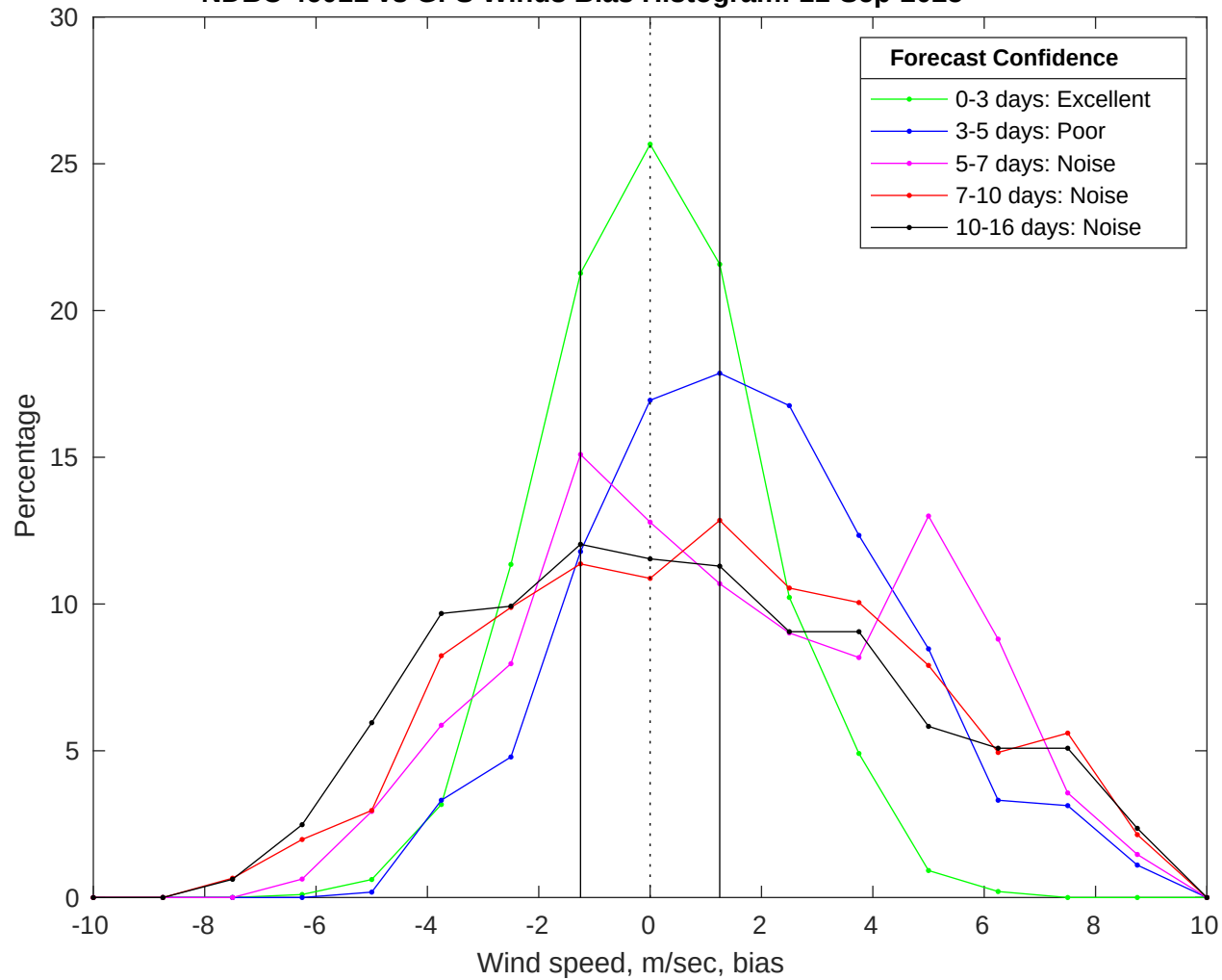
NDBC 46011 vs GFS Winds Bias Histogram: 11-Sep-2025
