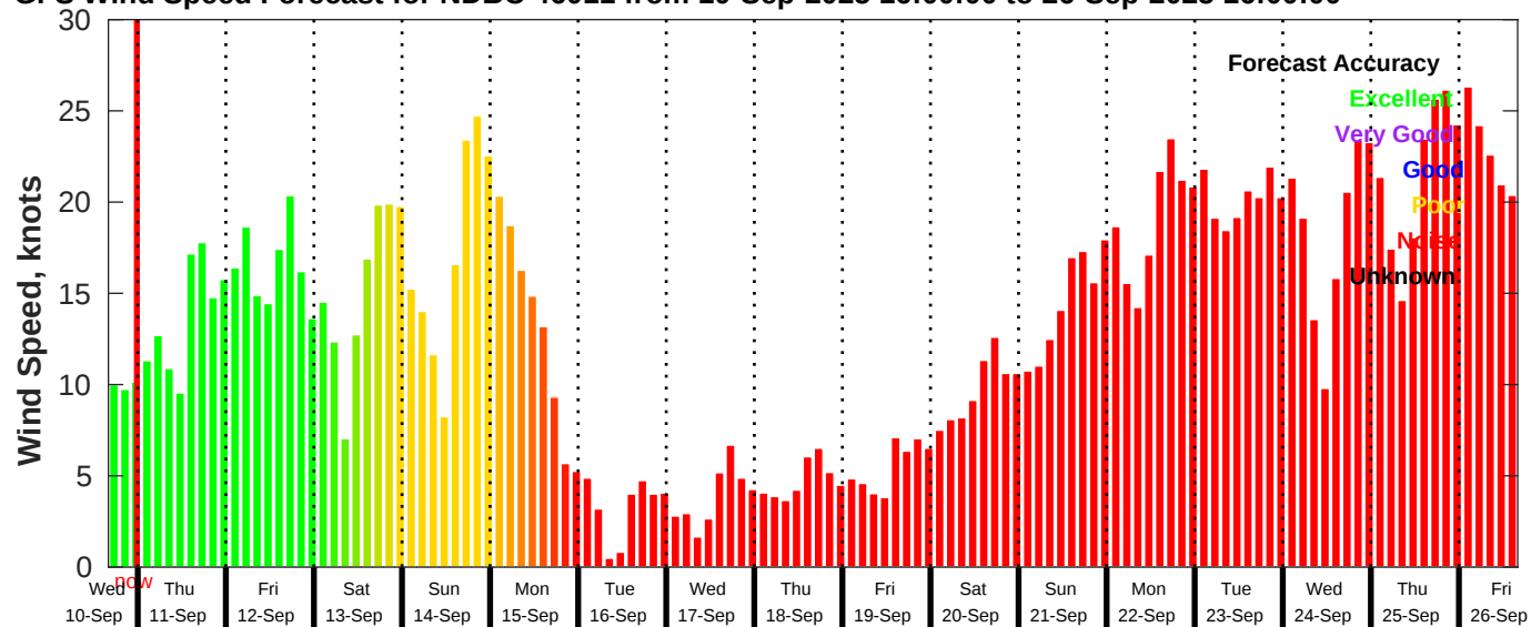
GFS Wind Speed Forecast for NDBC 46011 from 10-Sep-2025 16:00:00 to 26-Sep-2025 16:00:00
