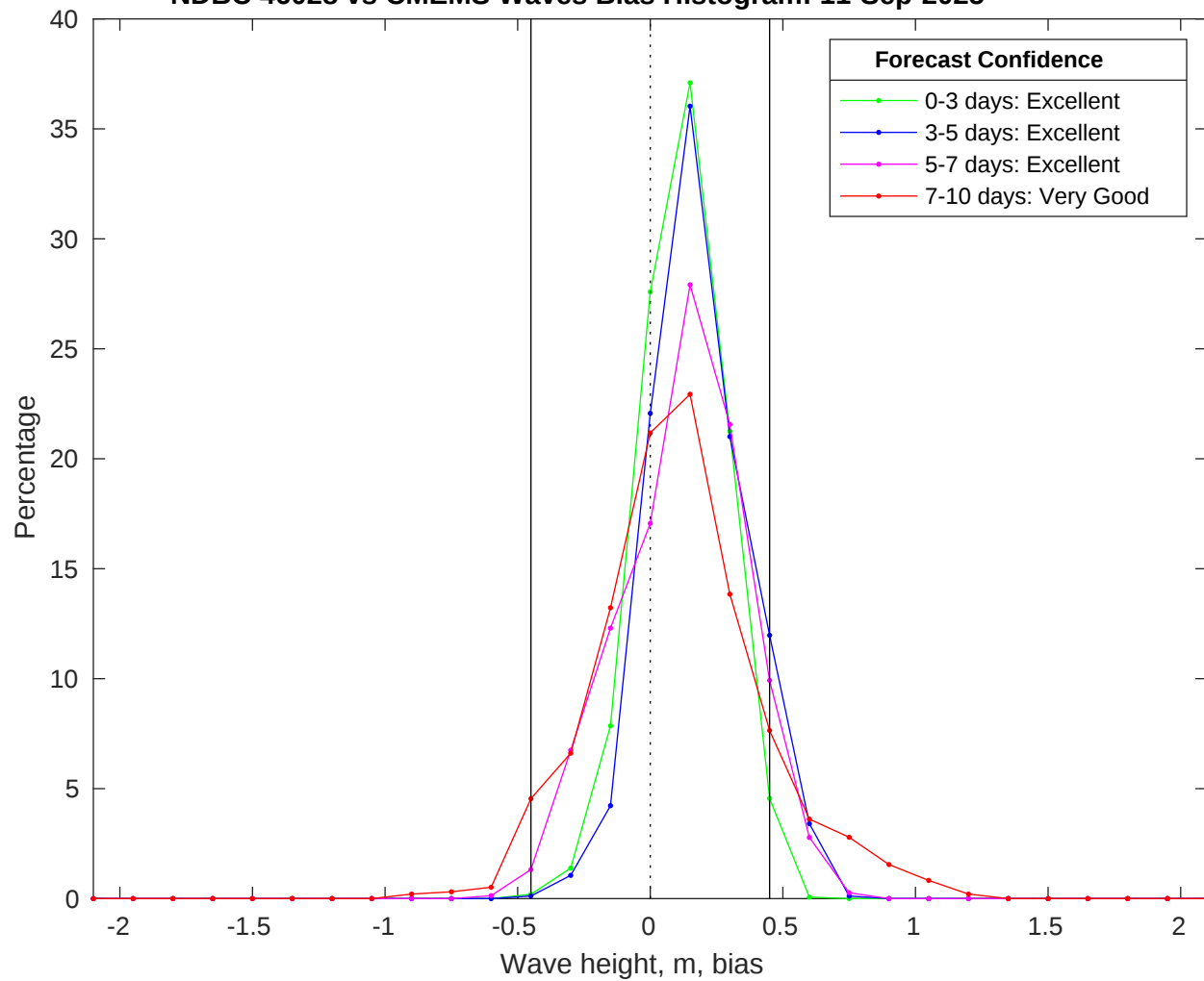
NDBC 46028 vs CMEMS Waves Bias Histogram: 11-Sep-2025
