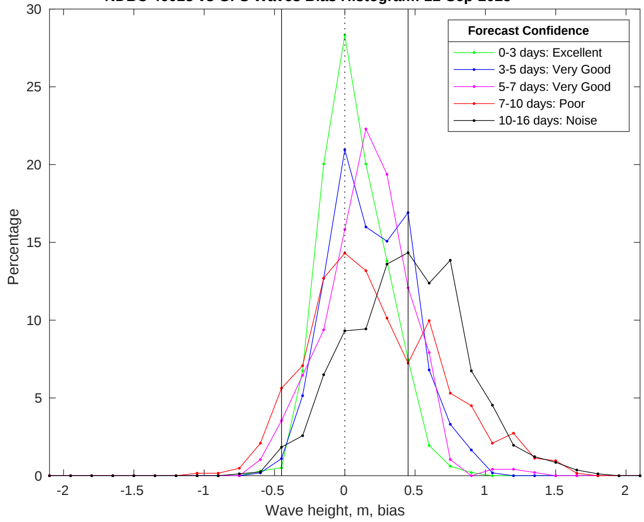
NDBC 46028 vs GFS Waves Bias Histogram: 11-Sep-2025
