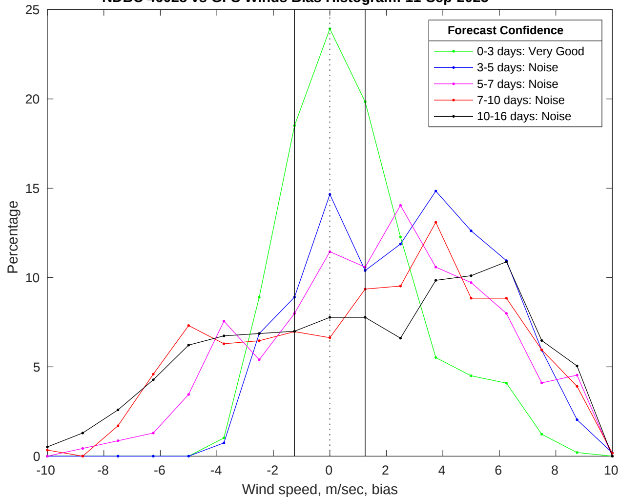
NDBC 46028 vs GFS Winds Bias Histogram: 11-Sep-2025
