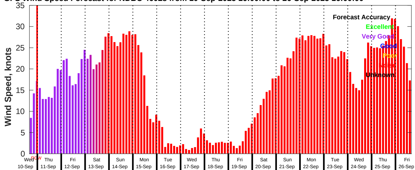
GFS Wind Speed Forecast for NDBC 46028 from 10-Sep-2025 16:00:00 to 26-Sep-2025 16:00:00
