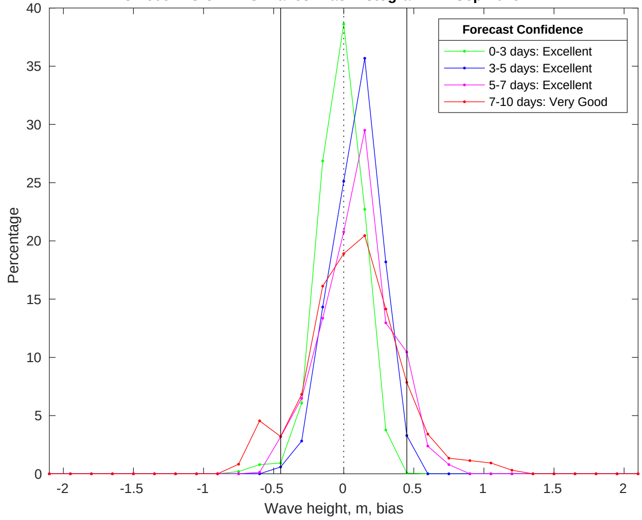
NDBC 46054 vs CMEMS Waves Bias Histogram: 11-Sep-2025
