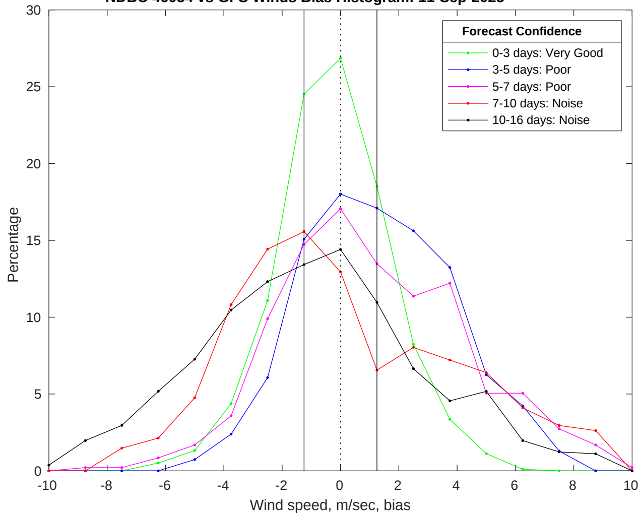
NDBC 46054 vs GFS Winds Bias Histogram: 11-Sep-2025
