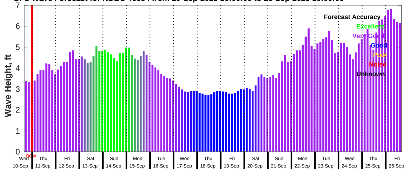
GFS Wave Forecast for NDBC 46054 from 10-Sep-2025 16:00:00 to 26-Sep-2025 16:00:00
