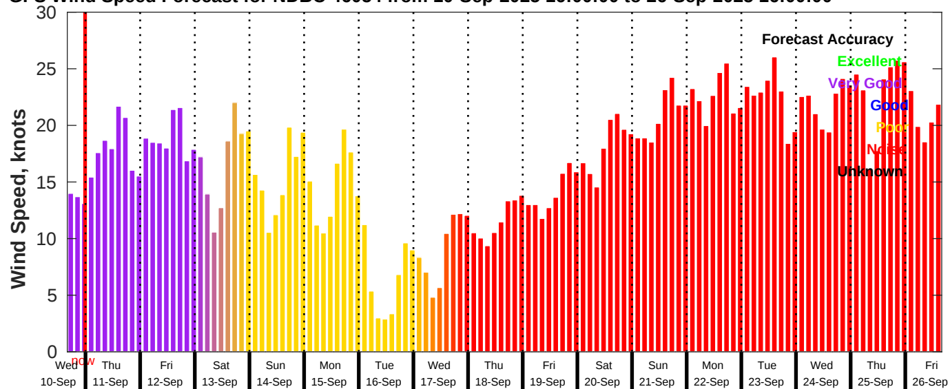
GFS Wind Speed Forecast for NDBC 46054 from 10-Sep-2025 16:00:00 to 26-Sep-2025 16:00:00
