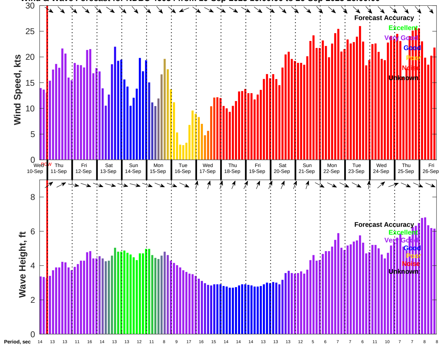
Wind & Wave Forecast for NDBC 46054 from 10-Sep-2025 16:00:00 to 26-Sep-2025 16:00:00
