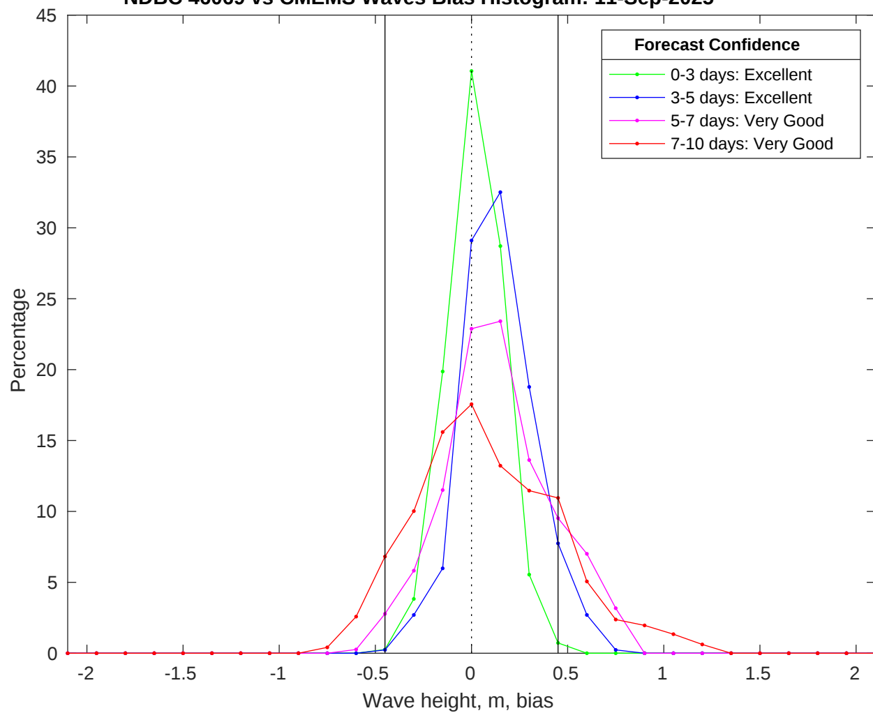
NDBC 46069 vs CMEMS Waves Bias Histogram: 11-Sep-2025
