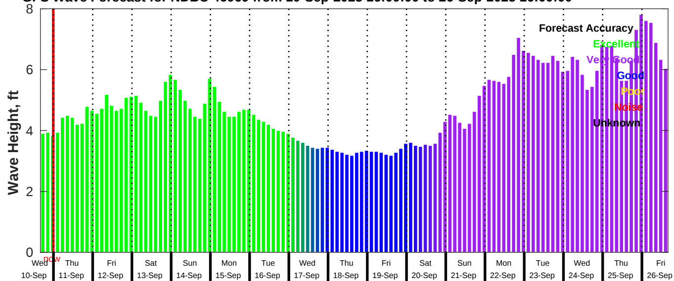
GFS Wave Forecast for NDBC 46069 from 10-Sep-2025 16:00:00 to 26-Sep-2025 16:00:00
