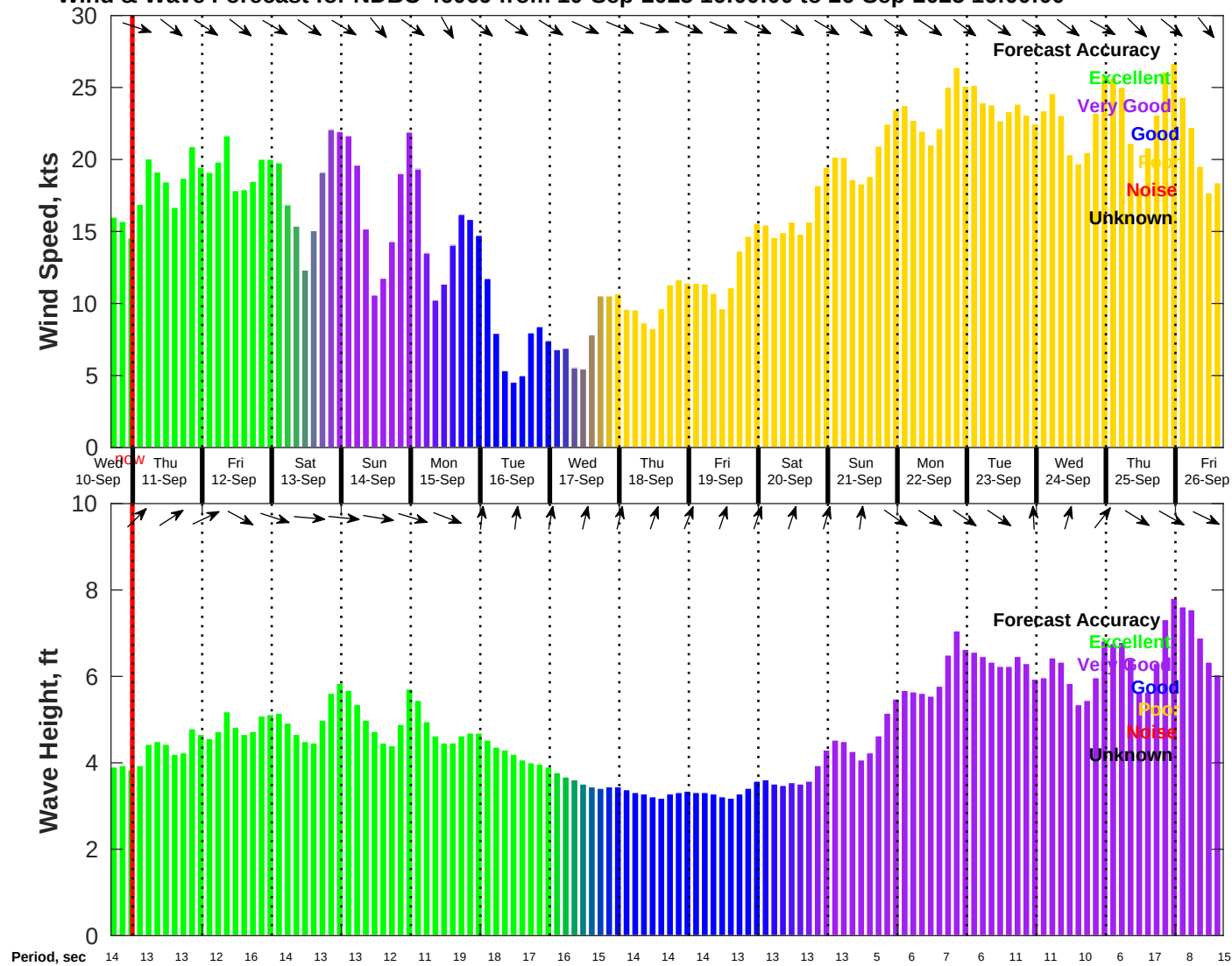
Wind & Wave Forecast for NDBC 46069 from 10-Sep-2025 16:00:00 to 26-Sep-2025 16:00:00
