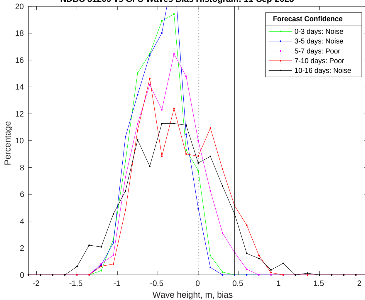
NDBC 51209 vs GFS Waves Bias Histogram: 11-Sep-2025
