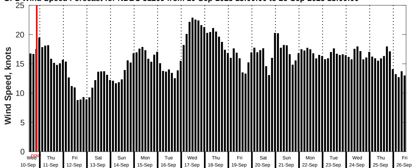
GFS Wind Speed Forecast for NDBC 51209 from 10-Sep-2025 13:00:00 to 26-Sep-2025 13:00:00
