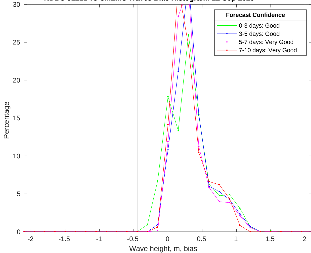
NDBC 51211 vs CMEMS Waves Bias Histogram: 11-Sep-2025
