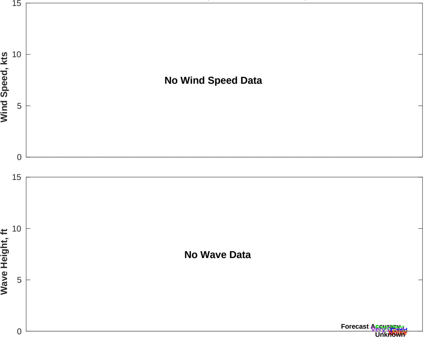
Wind & Wave Forecast for NDBC 51211 from 10-Sep-2025 14:00:00 to 26-Sep-2025 14:00:00
