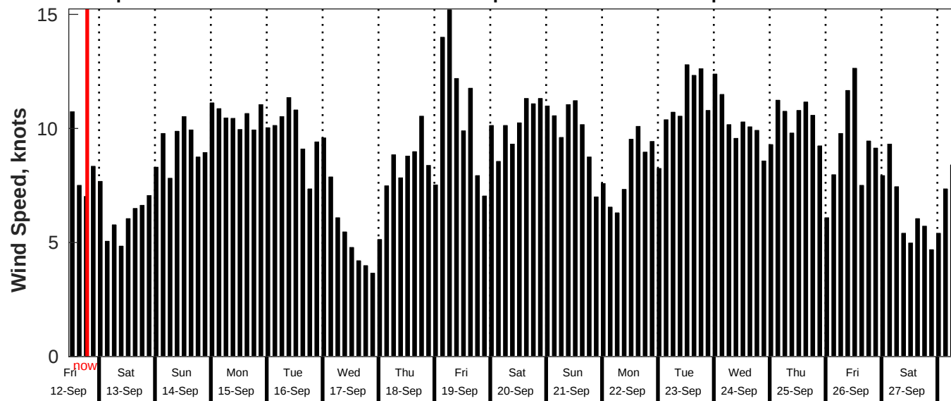
GFS Wind Speed Forecast for NDBC 52211 from 11-Sep-2025 11:00:00 to 27-Sep-2025 11:00:00
