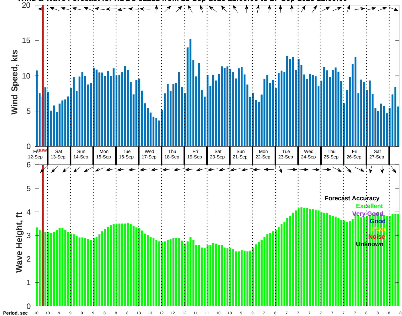
Wind & Wave Forecast for NDBC 52211 from 11-Sep-2025 11:00:00 to 27-Sep-2025 11:00:00
