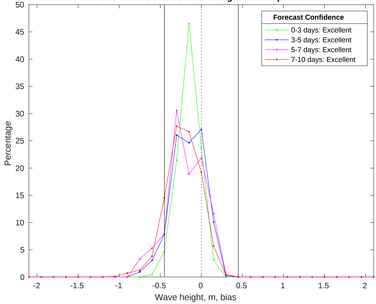
NDBC 52213 vs CMEMS Waves Bias Histogram: 11-Sep-2025
