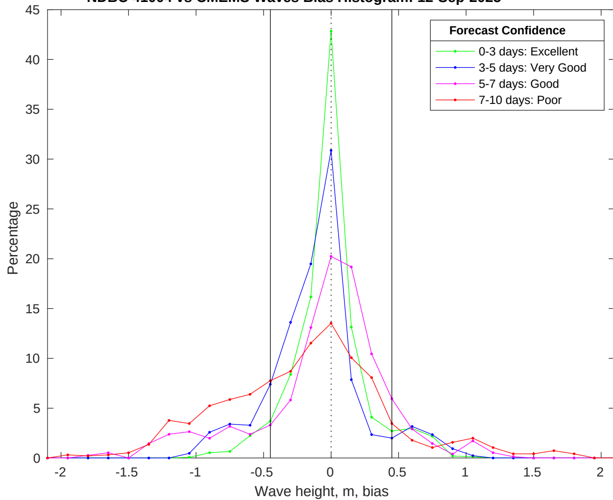
NDBC 41004 vs CMEMS Waves Bias Histogram: 12-Sep-2025
