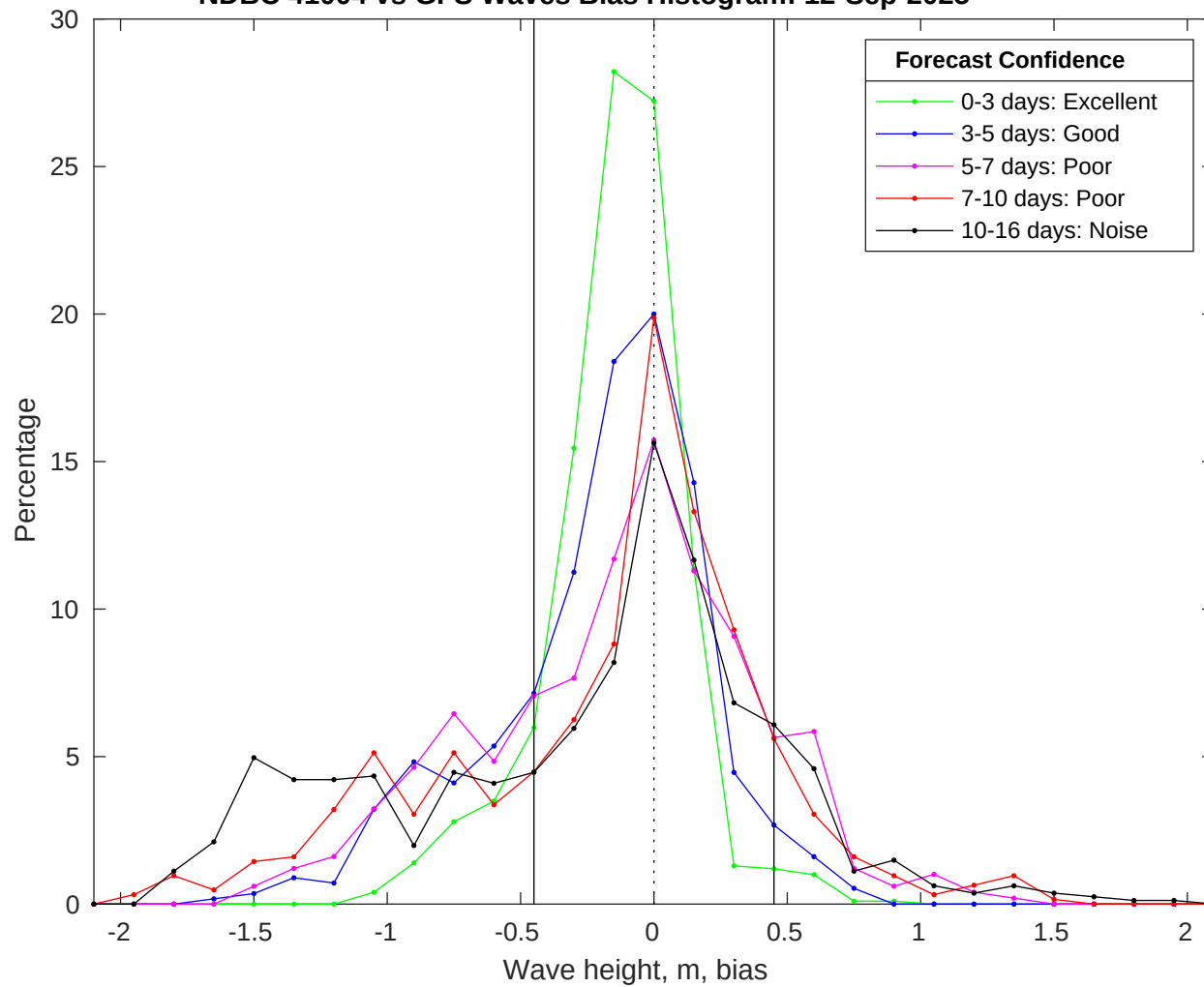
NDBC 41004 vs GFS Waves Bias Histogram: 12-Sep-2025
