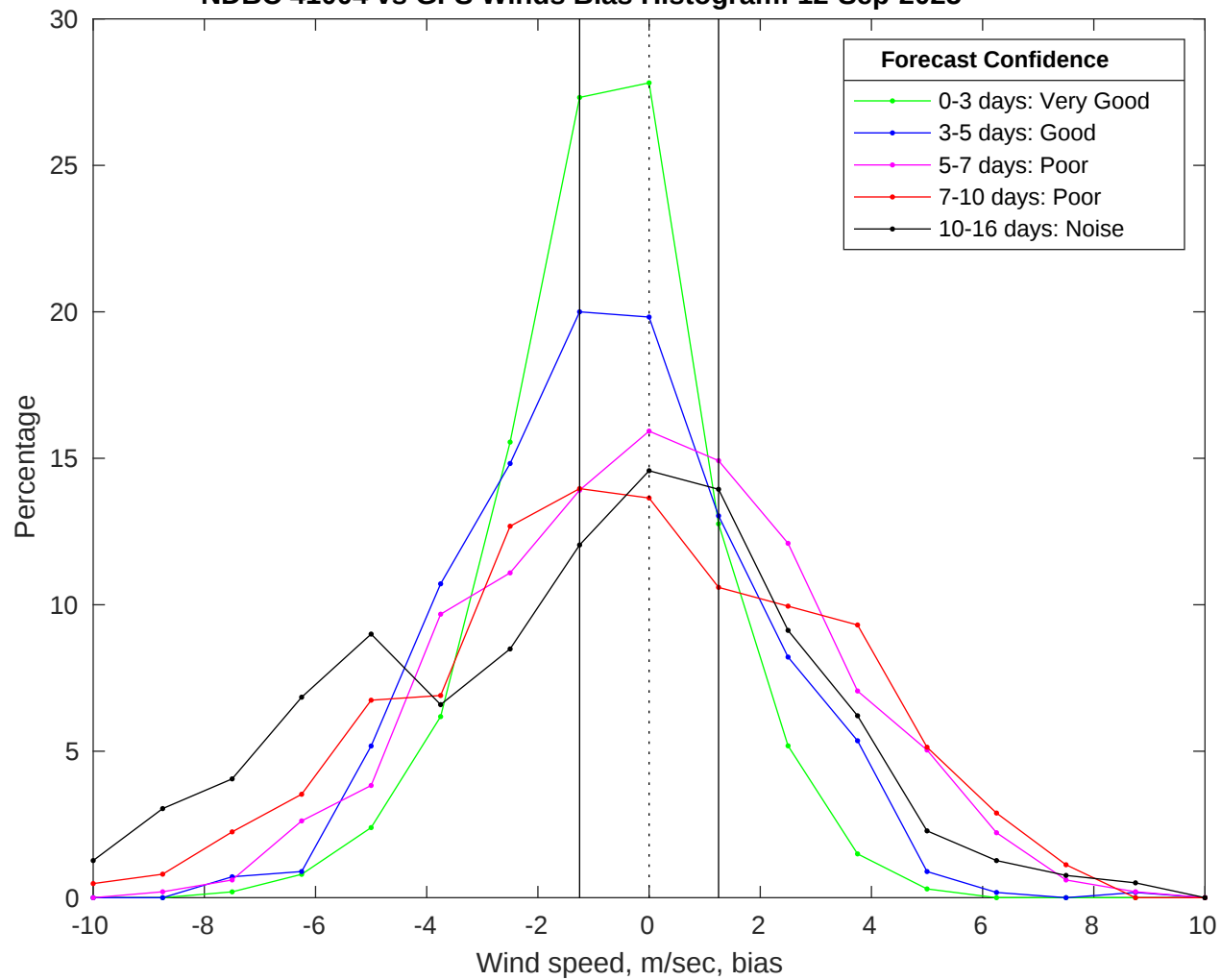
NDBC 41004 vs GFS Winds Bias Histogram: 12-Sep-2025
