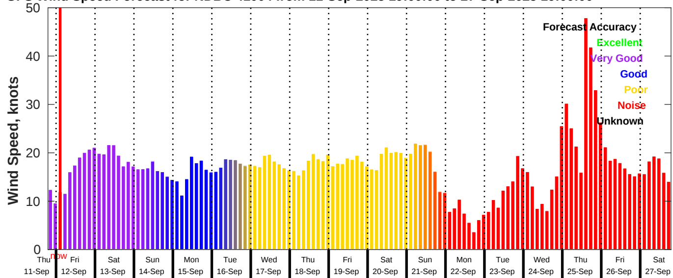
GFS Wind Speed Forecast for NDBC 41004 from 11-Sep-2025 19:00:00 to 27-Sep-2025 19:00:00
