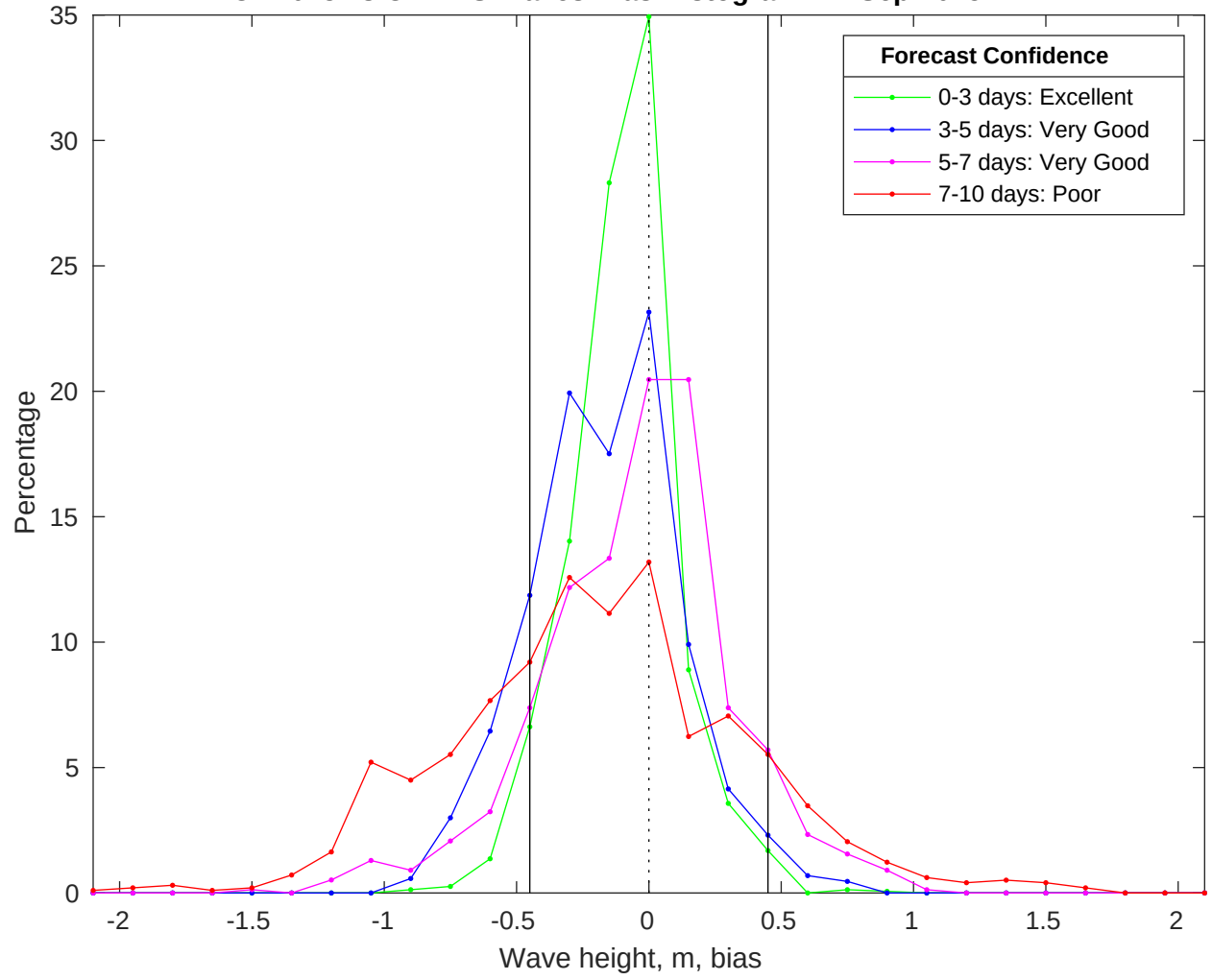
NDBC 41013 vs CMEMS Waves Bias Histogram: 12-Sep-2025
