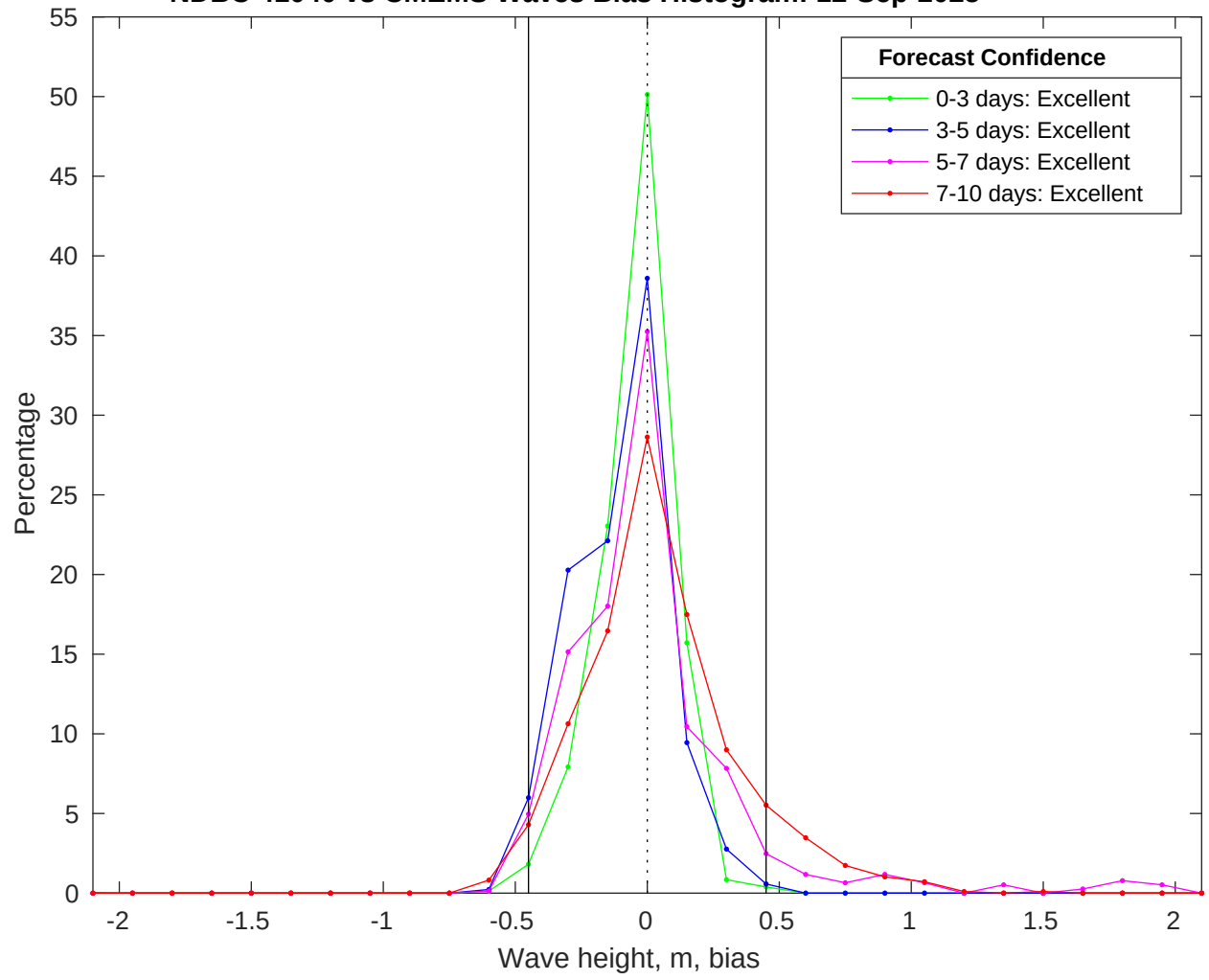
NDBC 41040 vs CMEMS Waves Bias Histogram: 12-Sep-2025
