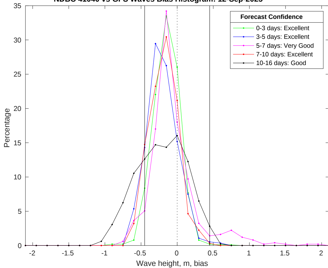
NDBC 41040 vs GFS Waves Bias Histogram: 12-Sep-2025
