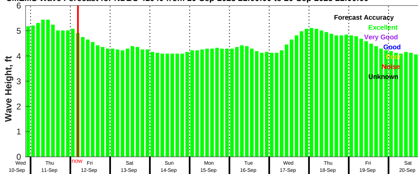
CMEMS Wave Forecast for NDBC 41040 from 10-Sep-2025 21:00:00 to 20-Sep-2025 21:00:00
