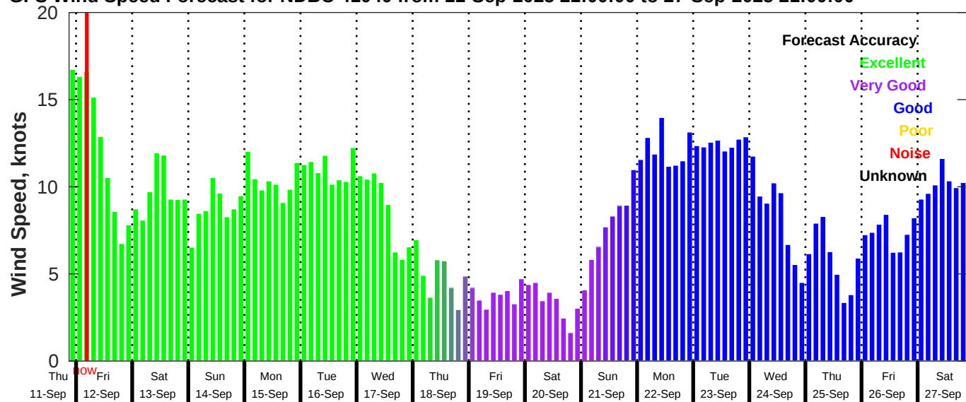
GFS Wind Speed Forecast for NDBC 41040 from 11-Sep-2025 21:00:00 to 27-Sep-2025 21:00:00
