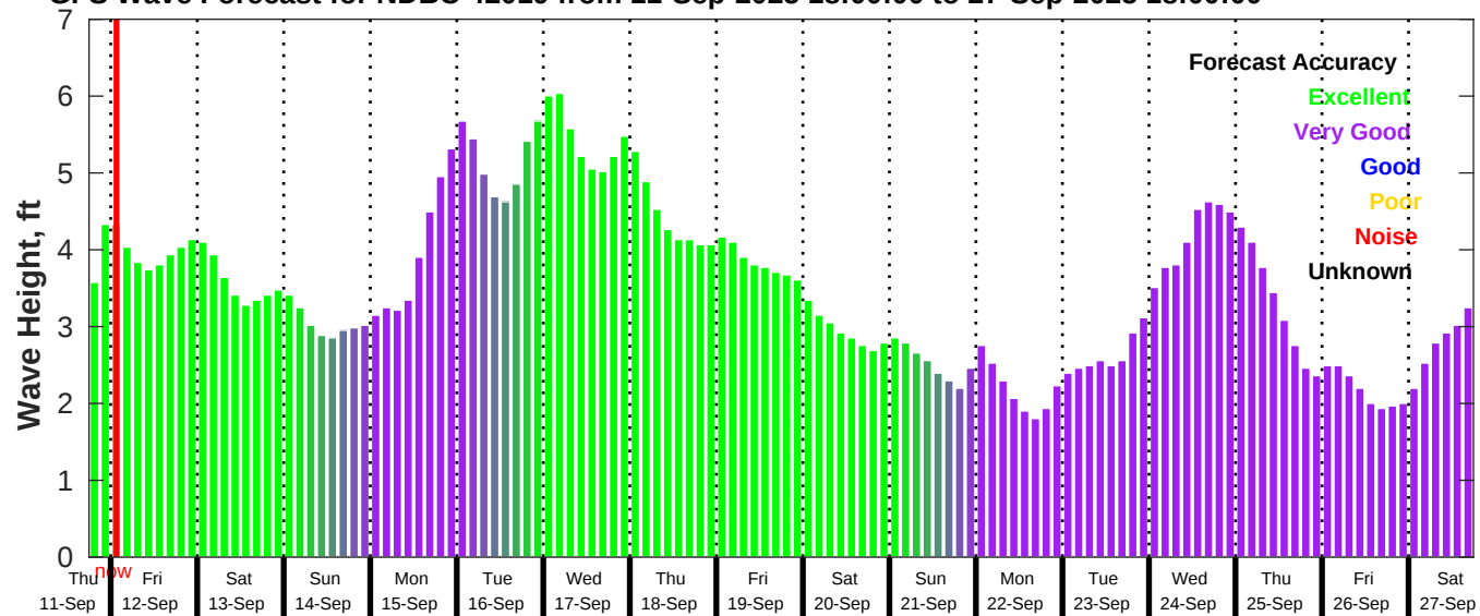
GFS Wave Forecast for NDBC 42019 from 11-Sep-2025 18:00:00 to 27-Sep-2025 18:00:00
