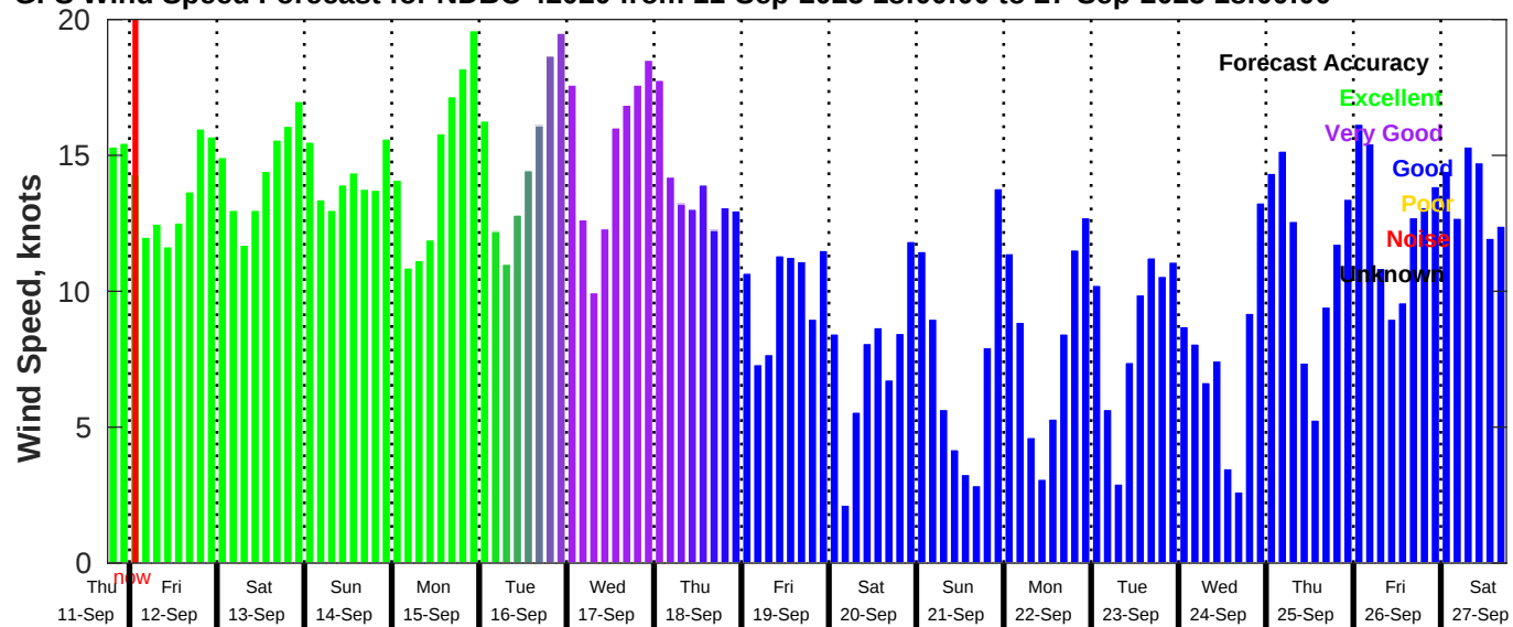
GFS Wind Speed Forecast for NDBC 42020 from 11-Sep-2025 18:00:00 to 27-Sep-2025 18:00:00
