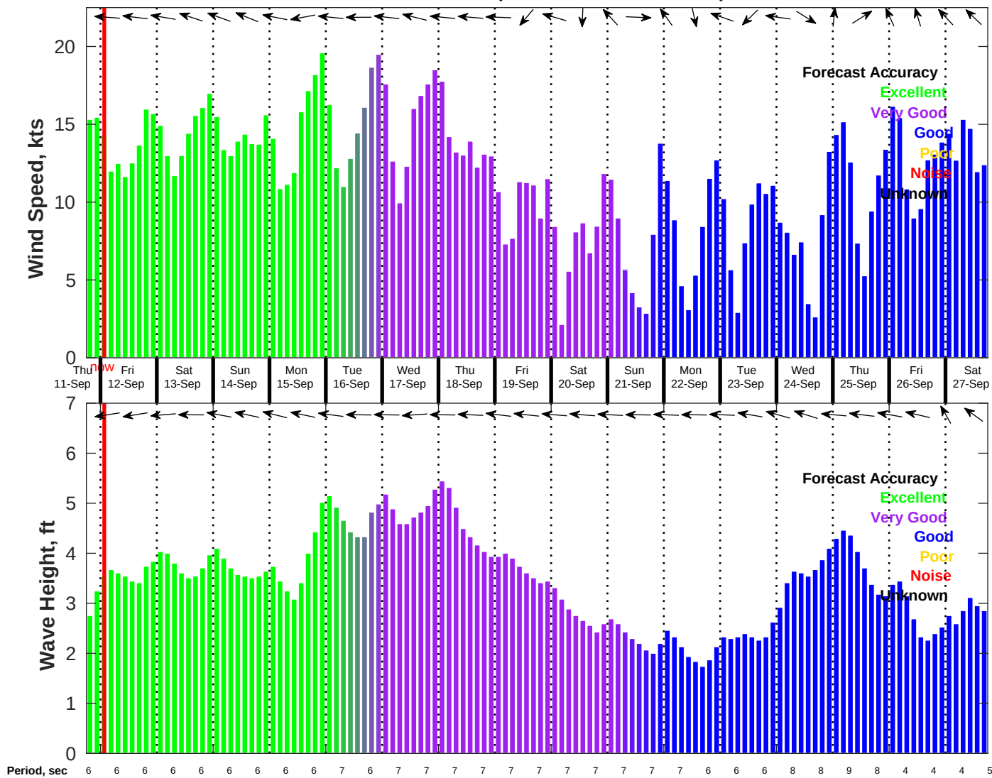
Wind & Wave Forecast for NDBC 42020 from 11-Sep-2025 18:00:00 to 27-Sep-2025 18:00:00
