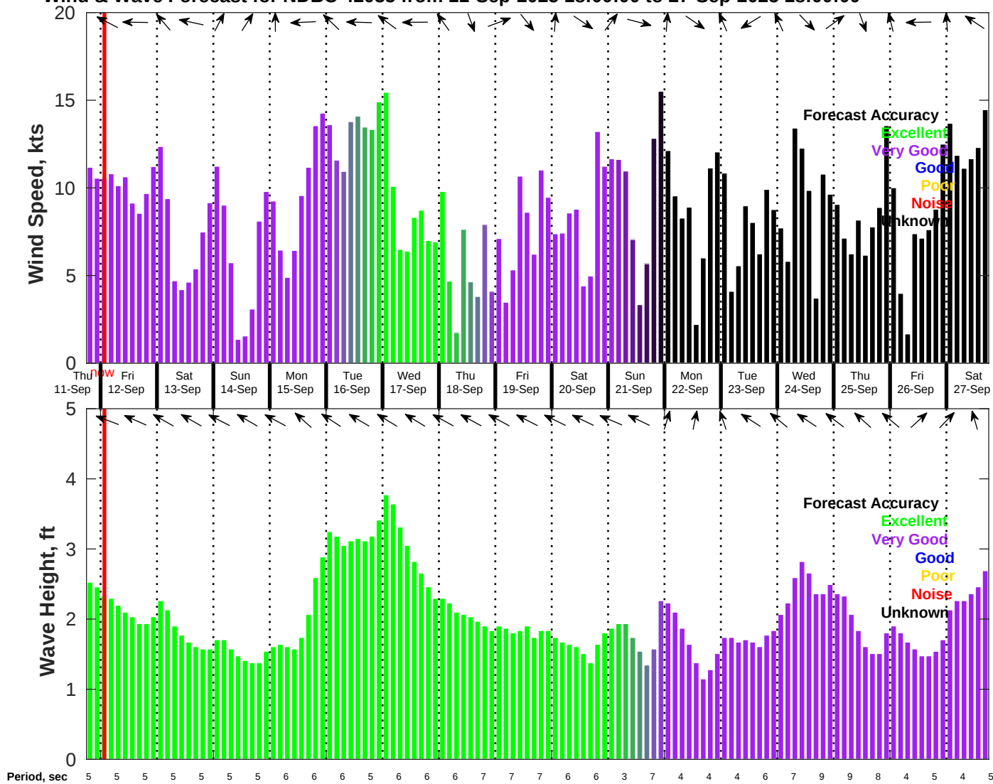
Wind & Wave Forecast for NDBC 42035 from 11-Sep-2025 18:00:00 to 27-Sep-2025 18:00:00
