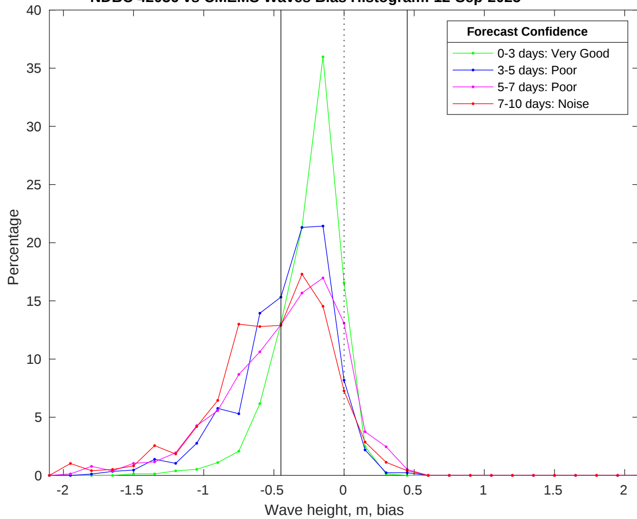
NDBC 42036 vs CMEMS Waves Bias Histogram: 12-Sep-2025
